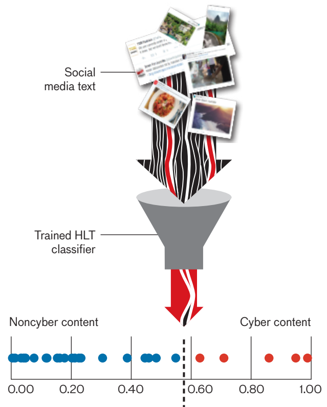
FIGURE 3. Text from a social media discussion is fed into a trained human language technology (HLT) classifier. The classifier then outputs the probability that the discussion is about cyber topics. This probability ranges from zero (not about cyber) to one (almost certainly about cyber). Output probabilities for different discussions are shown above, with a cyber content threshold (dashed line) that may be manually set by an analyst. An analyst would examine all discussions with probabilities above the threshold (red dots) and ignore remaining discussions with probabilities below the threshold (blue dots).
