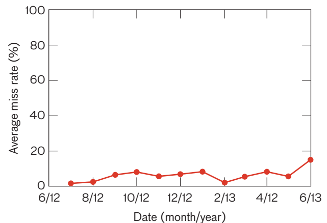
FIGURE 11. A logistic regression classifier was trained on Stack Exchange data before June 2012 and then tested every month after that for a year on new data. Despite the classifier not being retrained, its miss percentage increased little over the year and stayed below 20%.
